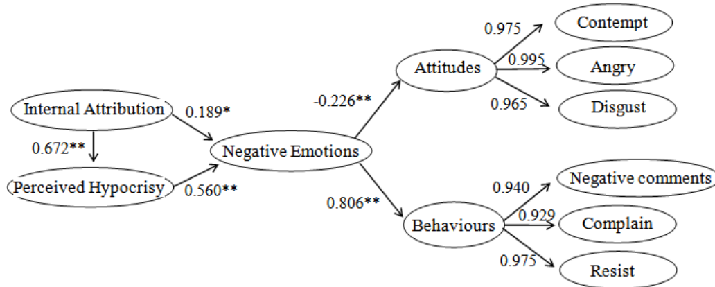
Figure. 2 path analysis results of structural equation model
